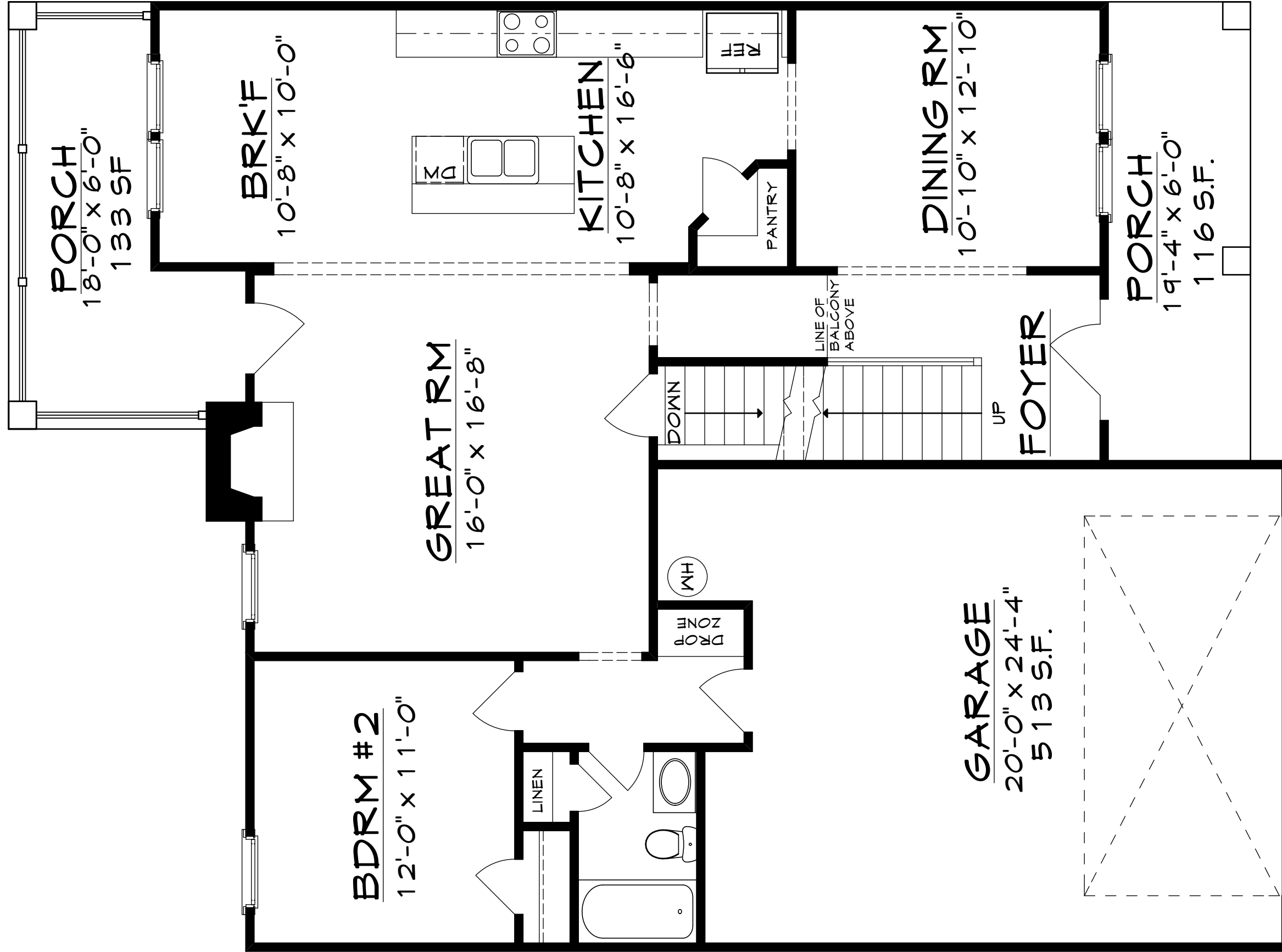
FIRST FLOOR PLAN 1150 SF HTD.
