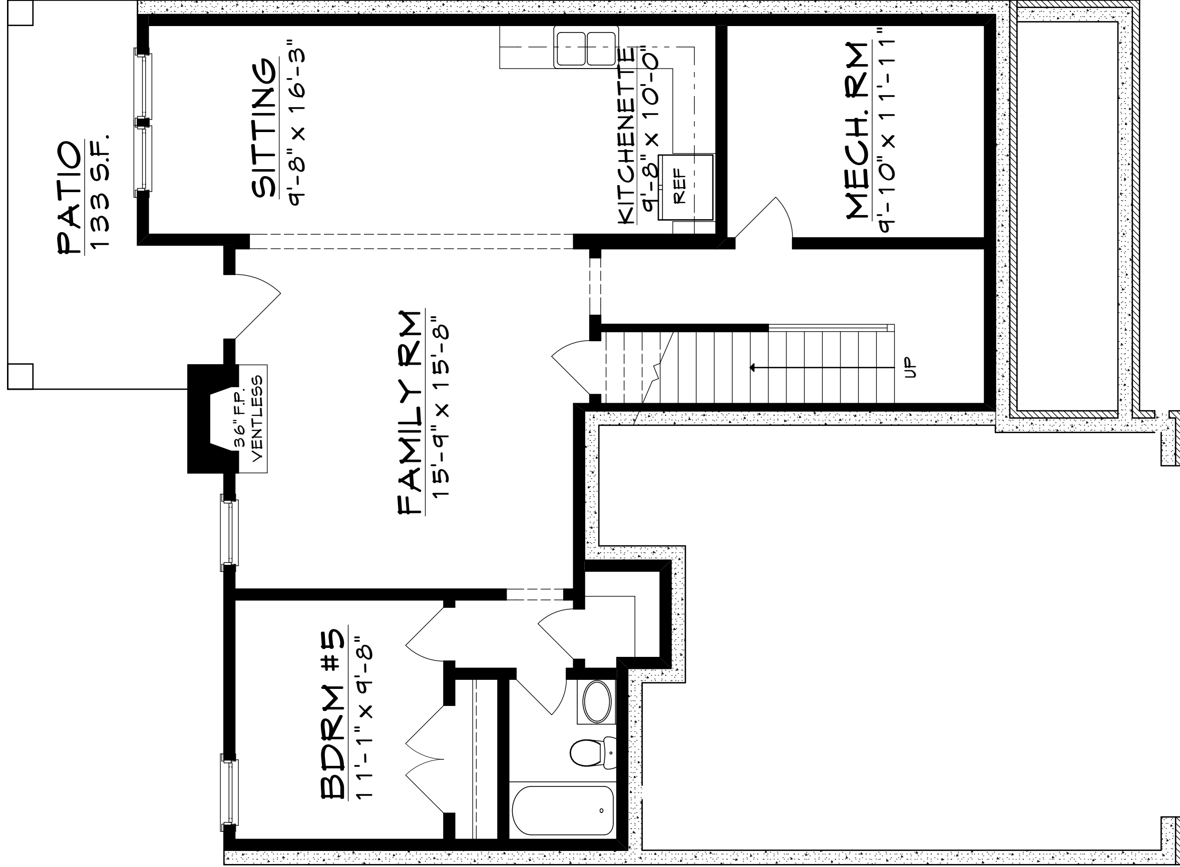
BASEMENT PLAN 1074 SF HTD.
